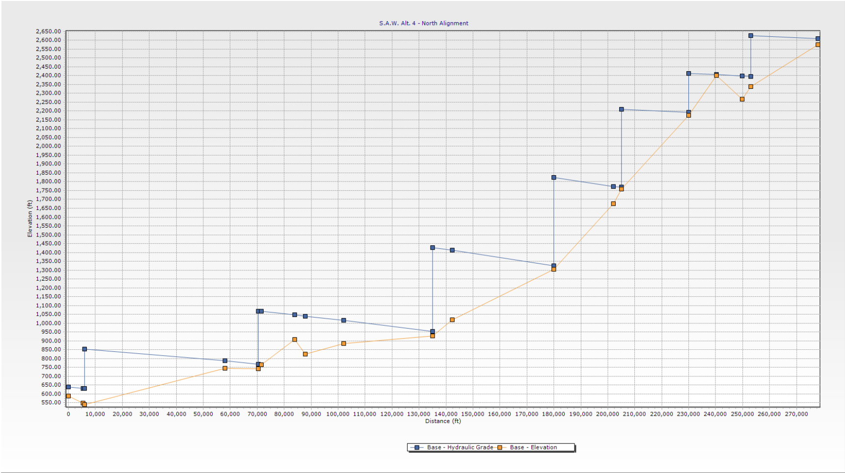
Exhibit 11 - SAW Alternative 4 - Profile of North Alignment
