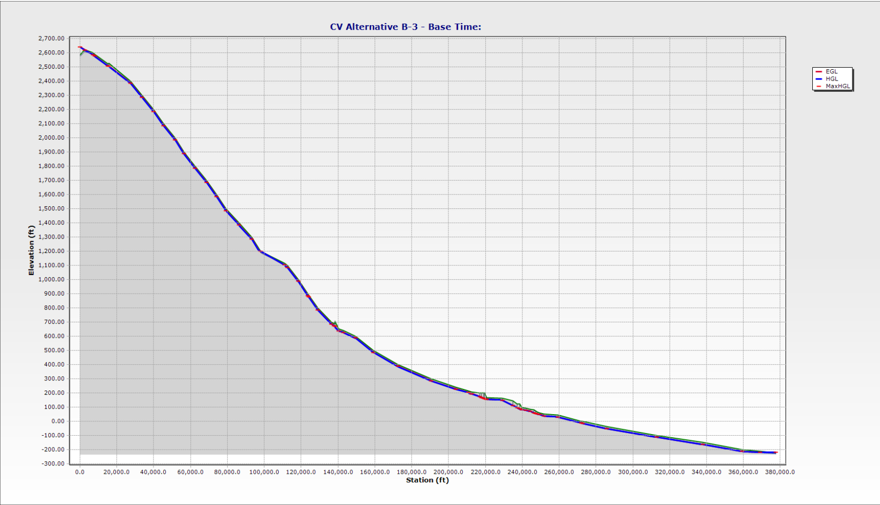
Exhibit 17 - CV Alternative B-3 Profile
